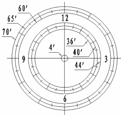
Figure 13. Polar scope dial
