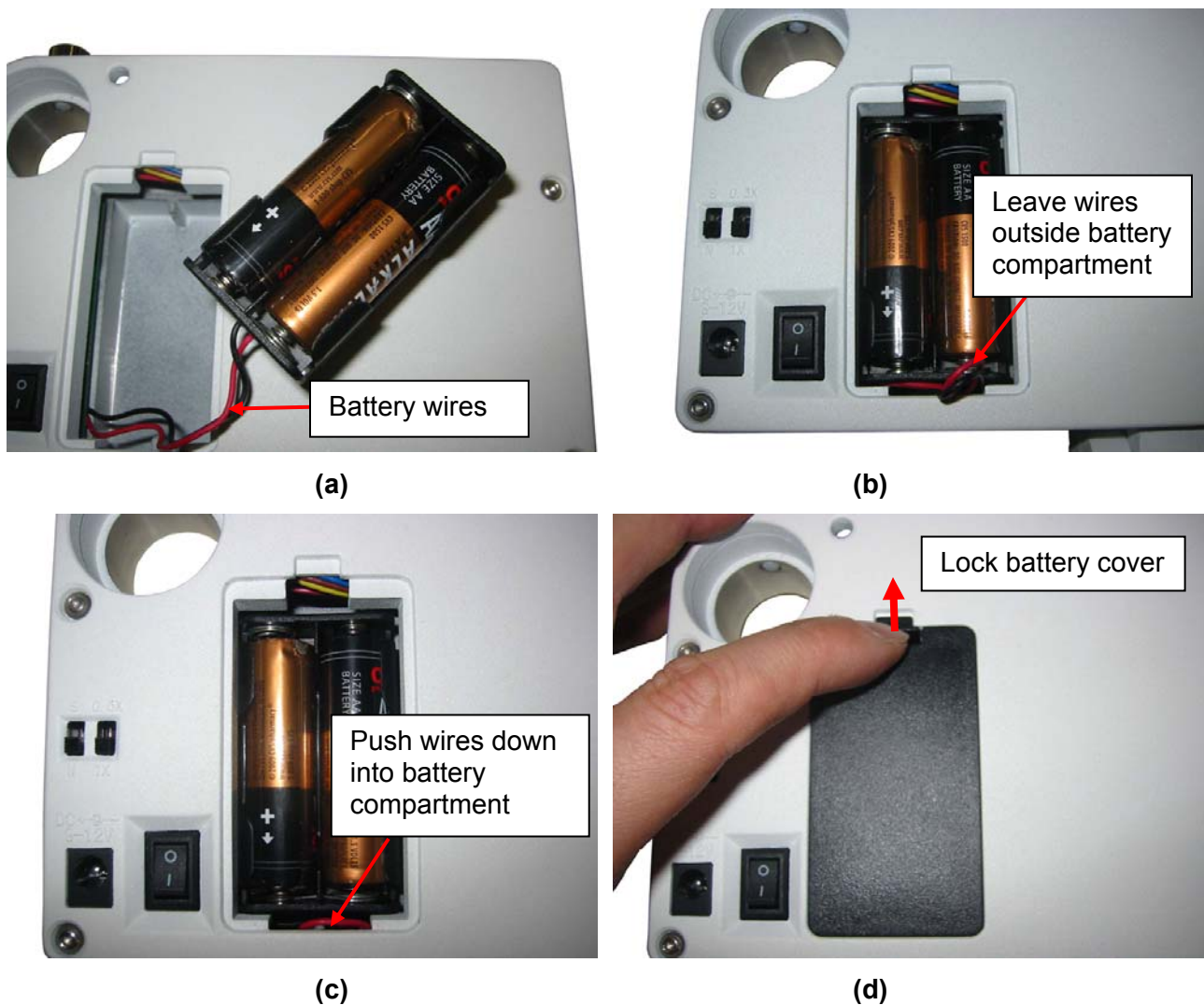
Figure 5. Install batteries
