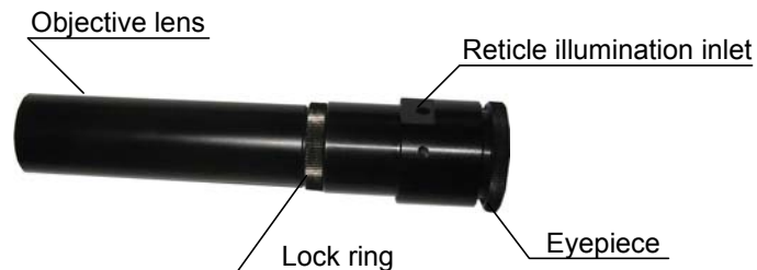
Figure 10. AccuAligning™ dark field illuminated polar scope
